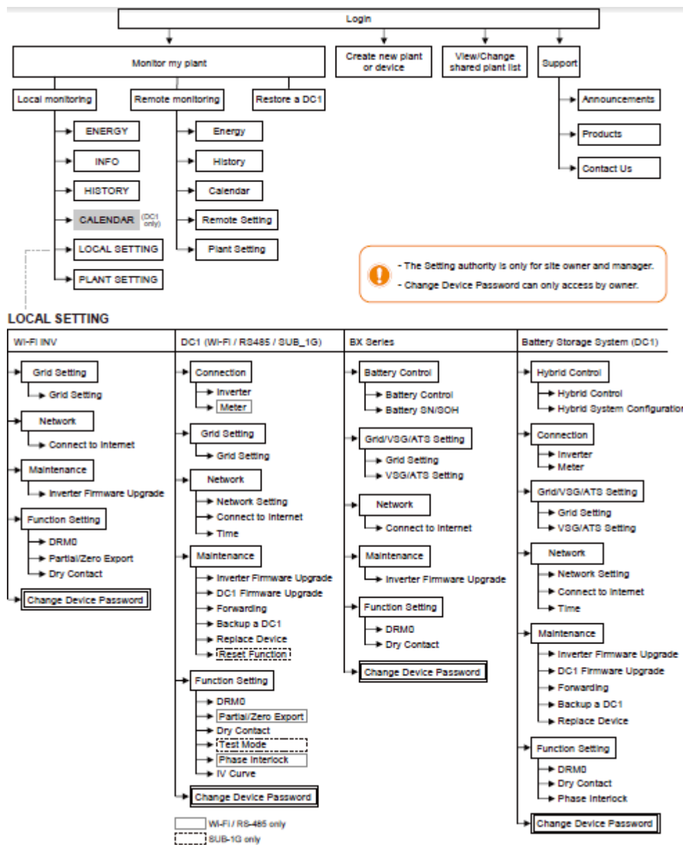
App Structure
